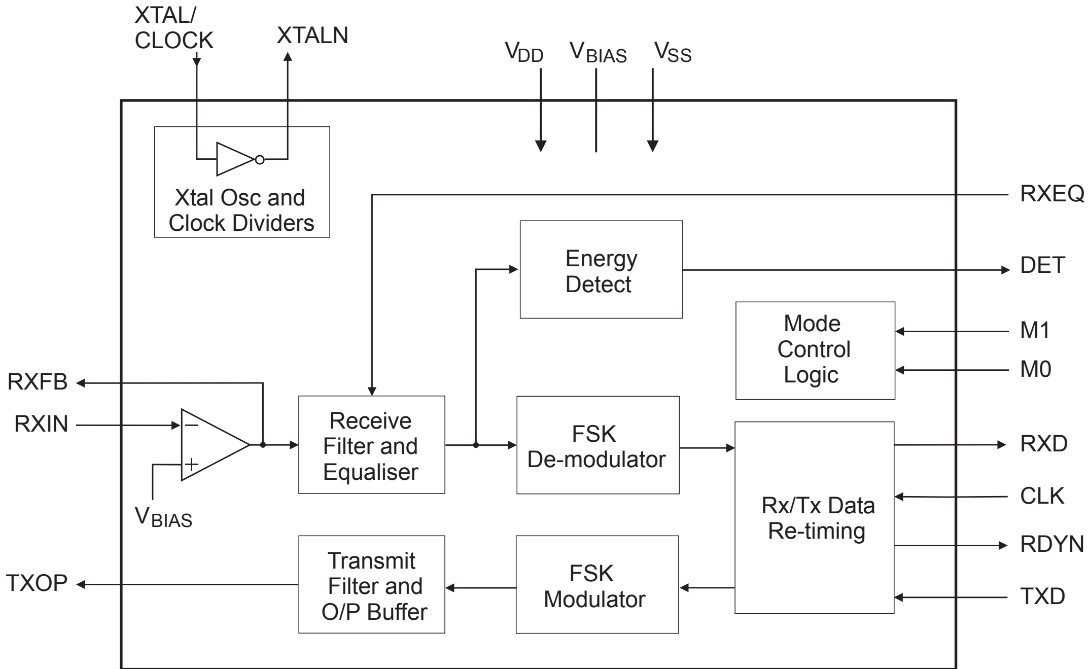
FX/MX604 Block Diagram
