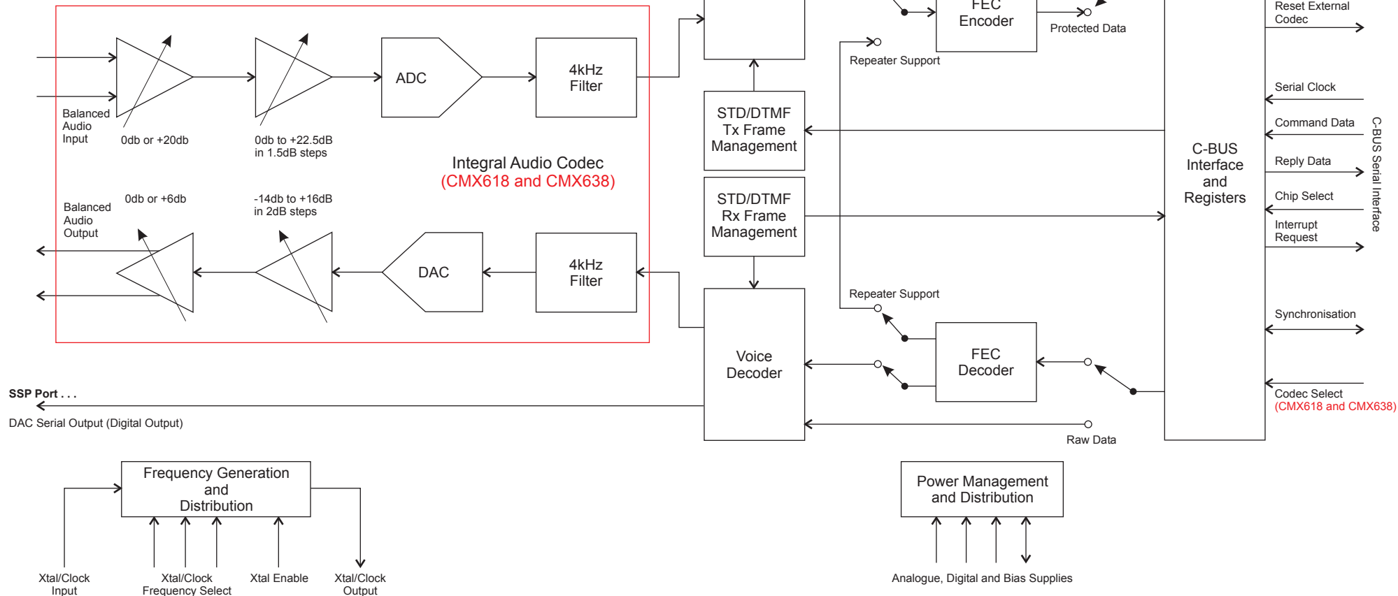
CMX6x8 Block Diagram
