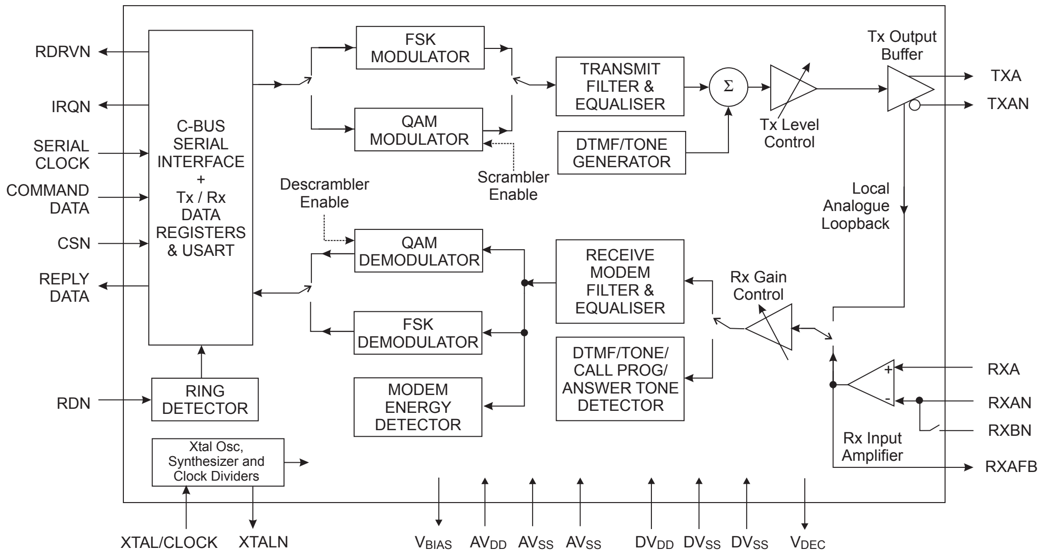
CMX869B Block Diagram
