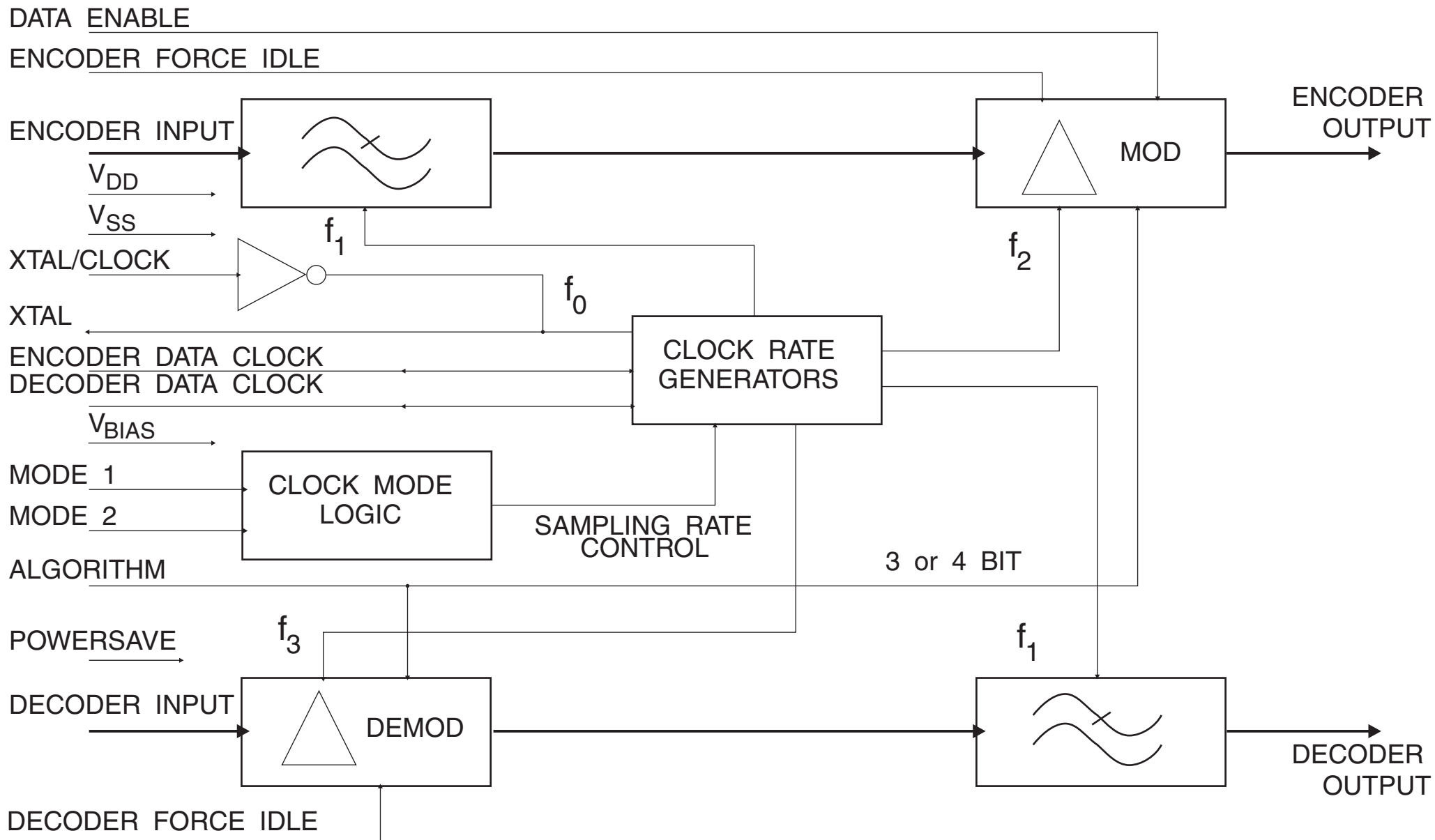
CMX639 Block Diagram
