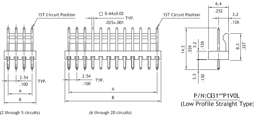
(2 through 5 circuits)
