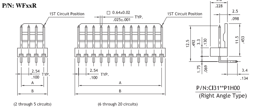
(2 through 5 circuits)
