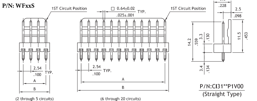
(2 through 5 circuits)
