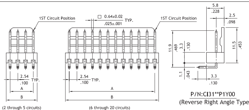
(2 through 5 circuits)
