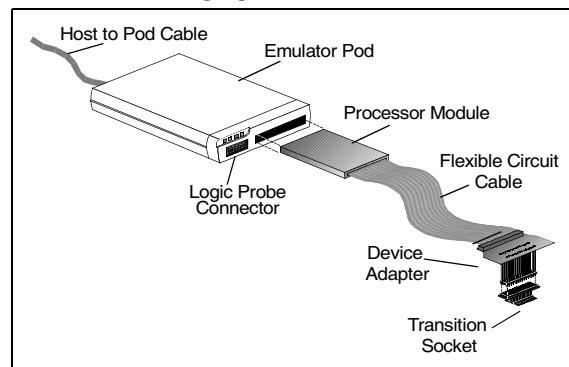
FIGURE 2-1: MPLAB ICE EMULATOR SYSTEM
