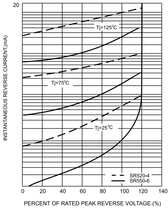
FIG.3-TYPICAL REVERSE CHARACTERISTICS
