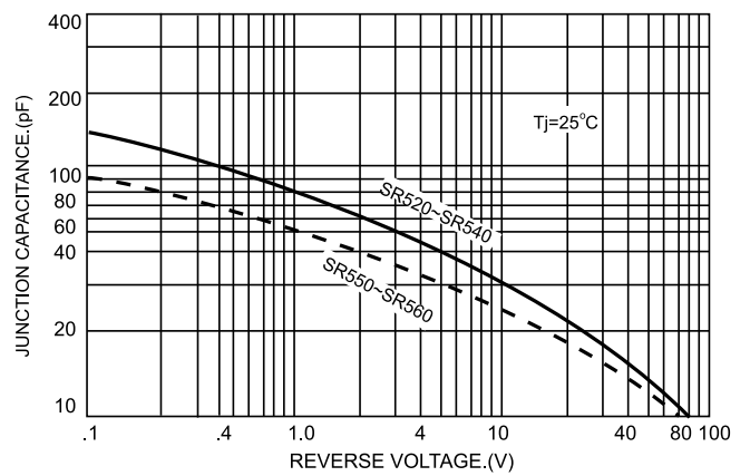
FIG.5-TYPICAL JUNCTION CAPACITANCE
