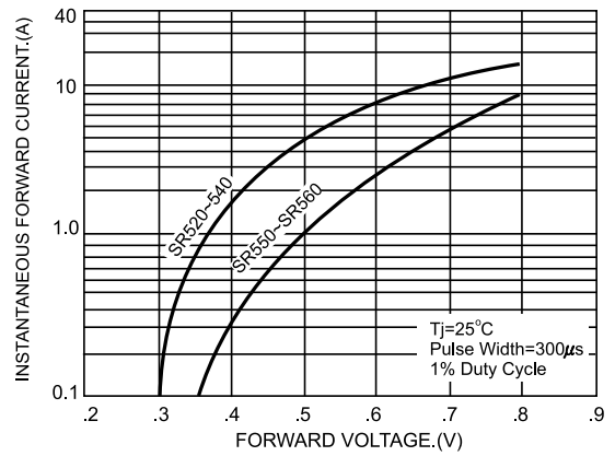
FIG.4-TYPICAL FORWARD CHARACTERISTICS
