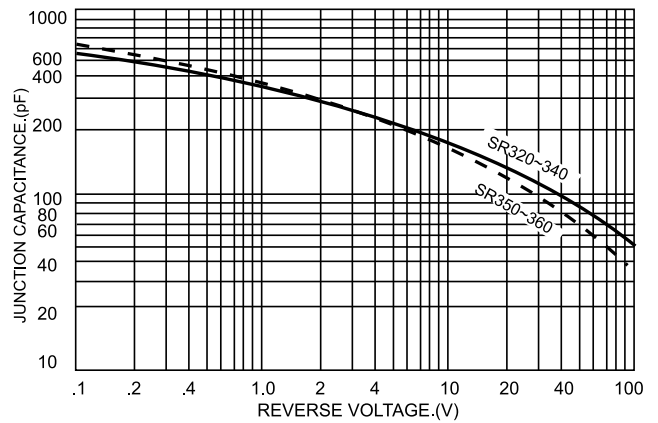
FIG.4-TYPICAL JUNCTION CAPACITANCE
