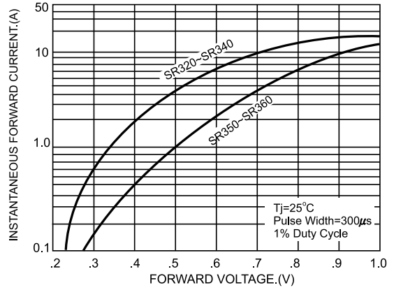
FIG.2-TYPICAL FORWARD CHARACTERISTICS
