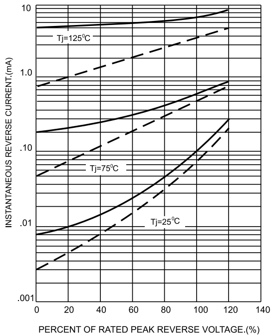
FIG.3-TYPICAL REVERSE CHARACTERISTICS
