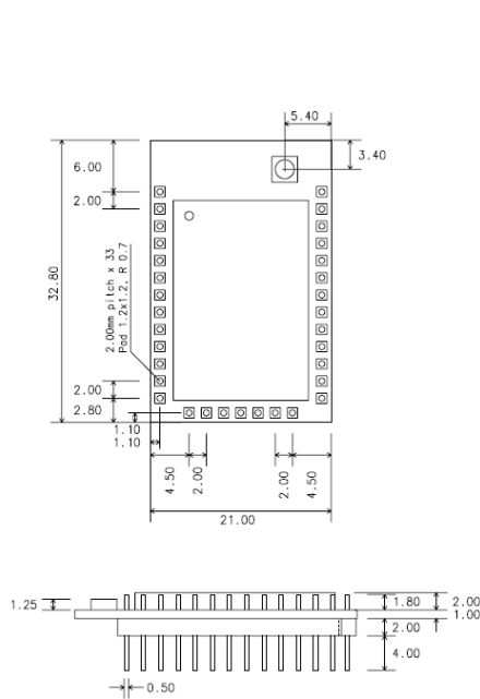
Figure 1-3 ProBee-ZE20SDU
