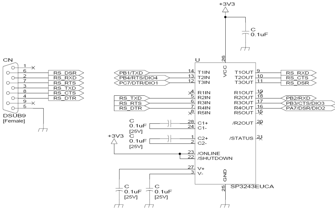
Figure 5-3 RS232 Serial
