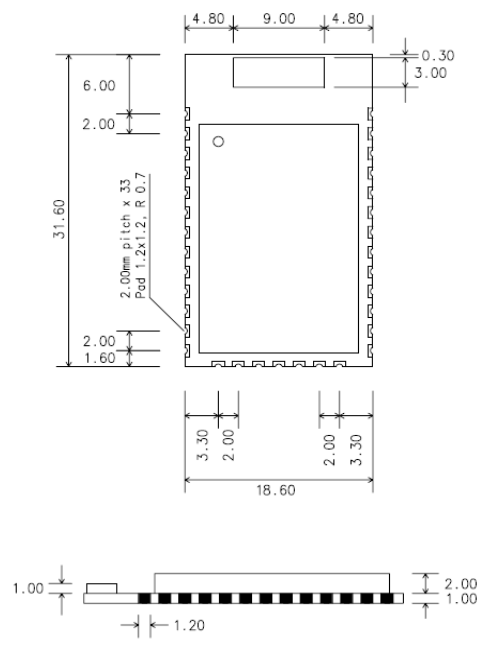
Figure 1-7 ProBee-ZE20SSC
