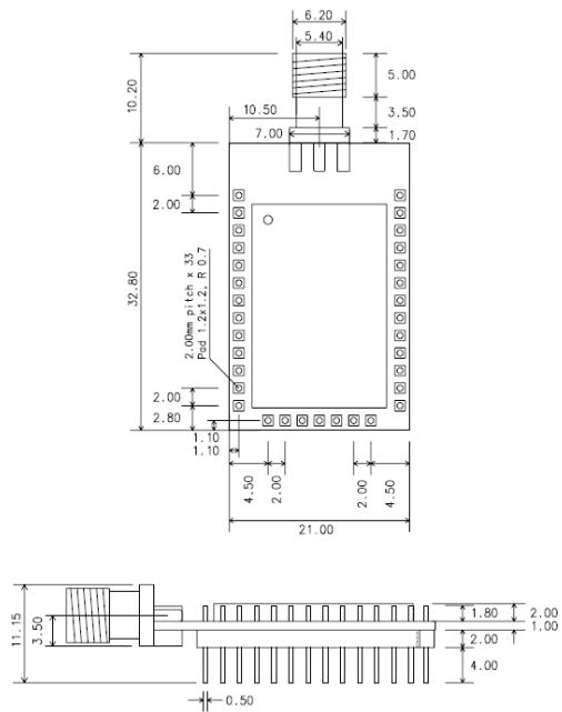
Figure 1-4 ProBee-ZE20SDS
