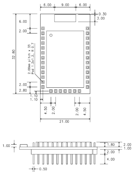
Figure 1-5 ProBee-ZE20SDC
