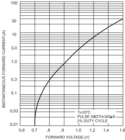
FIG.3-TYPICAL FORWARD CHARACTERISTICS
