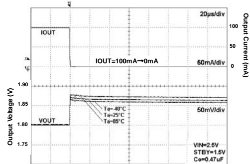
Fig 17. Load Response
