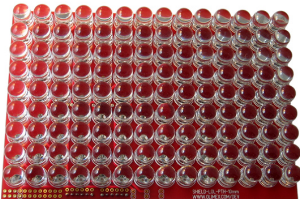
SHIELD-LOL-10MM
