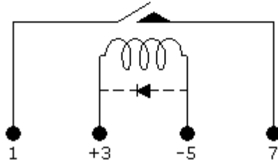
Wiring diagram (Top View)
