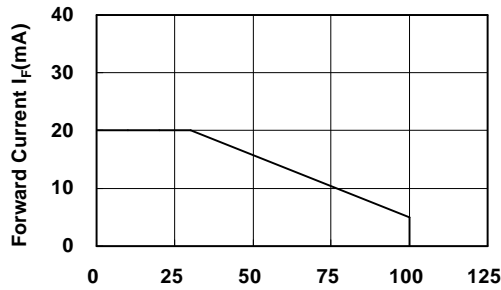
FIG3-26. FORWARD CURRENT VS. AMBLENT TEMPERATURE
