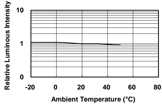
FIG4. LUMINOUS INTENSITY VS. AMUBIENT TEMPERATURE
