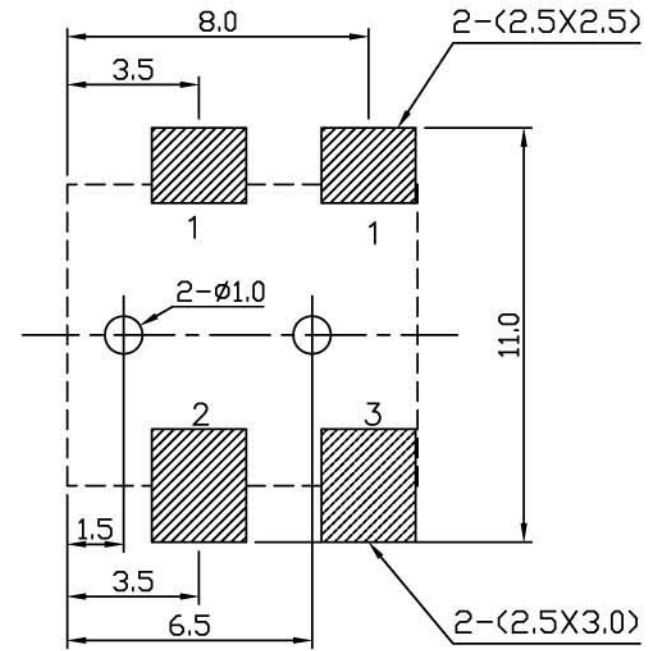
T:1.6 Dimensions of PC board holes
