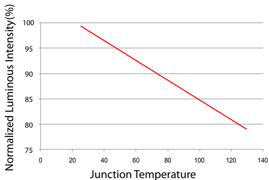
Junction Temperature vs. Luminous Intensity for PLCC 5630 series
