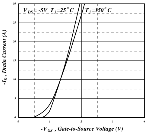
Fig 11. Transfer Characteristics
