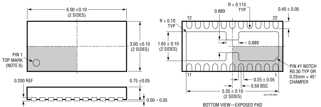
BOTTOM VIEW—EXPOSED PAD
