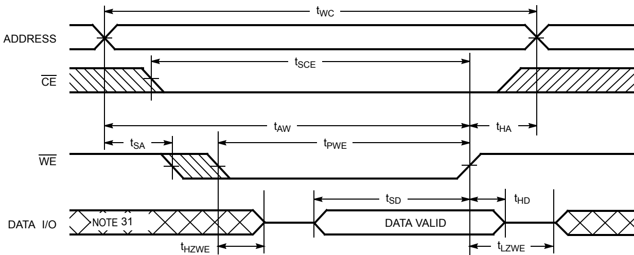
Figure 7. Write Cycle No. 3 ( \overline{WE} Controlled, \overline{OE} LOW) [30]
