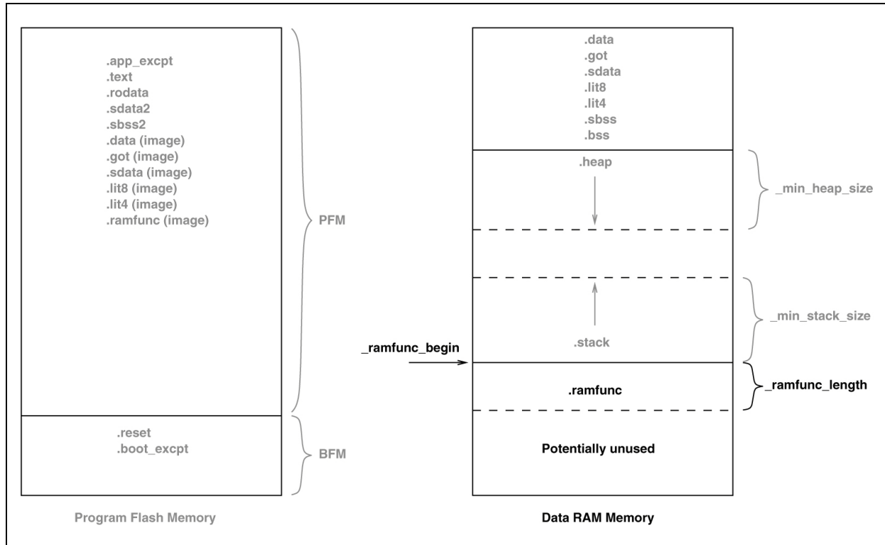
FIGURE 14-4: BUS MATRIX INITIALIZATION
