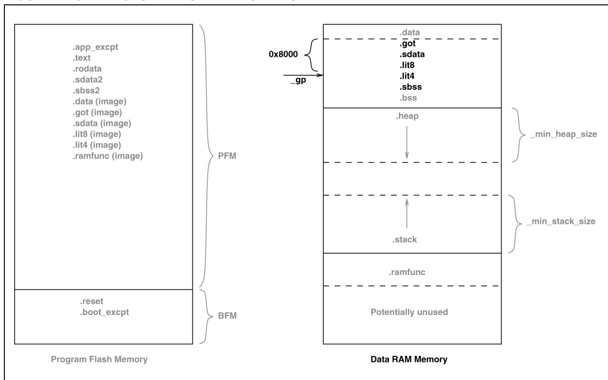
FIGURE 14-3: GLOBAL POINTER LOCATION
