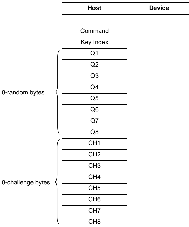
Figure 20. Verify Crypto Command Functional Description
